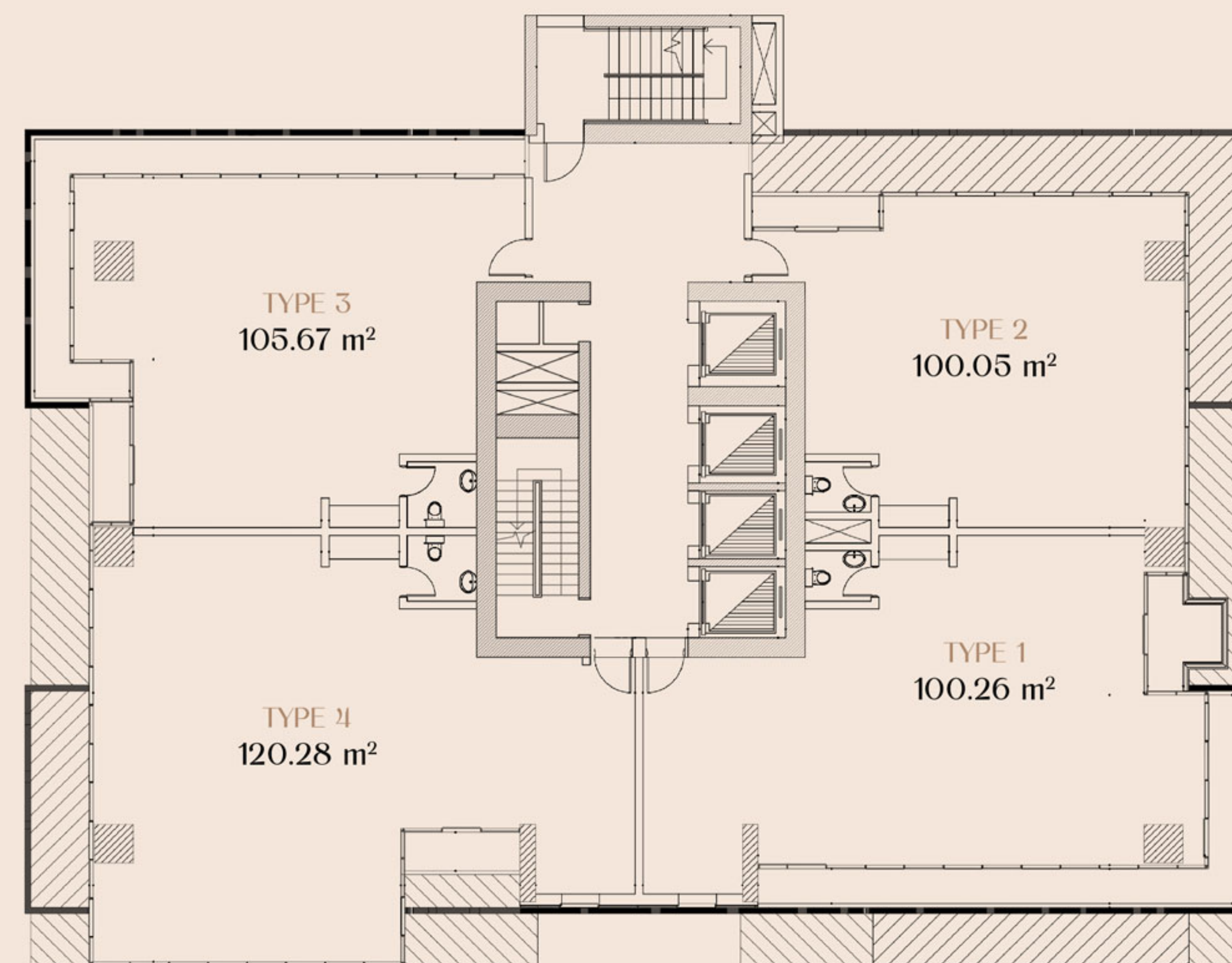
22 nd , 26 th FLOOR
