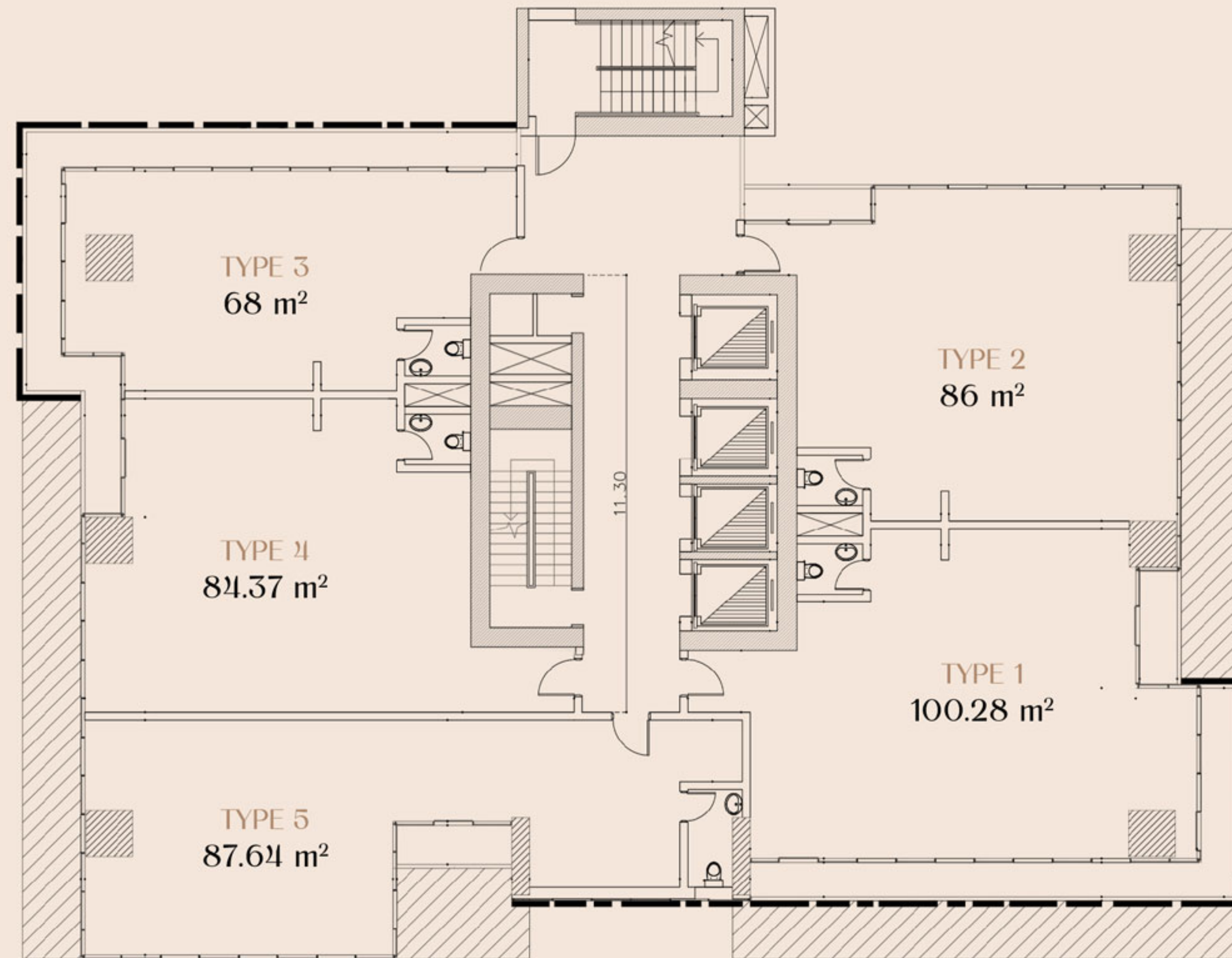
2 nd , 3 rd , 4 th FLOOR
