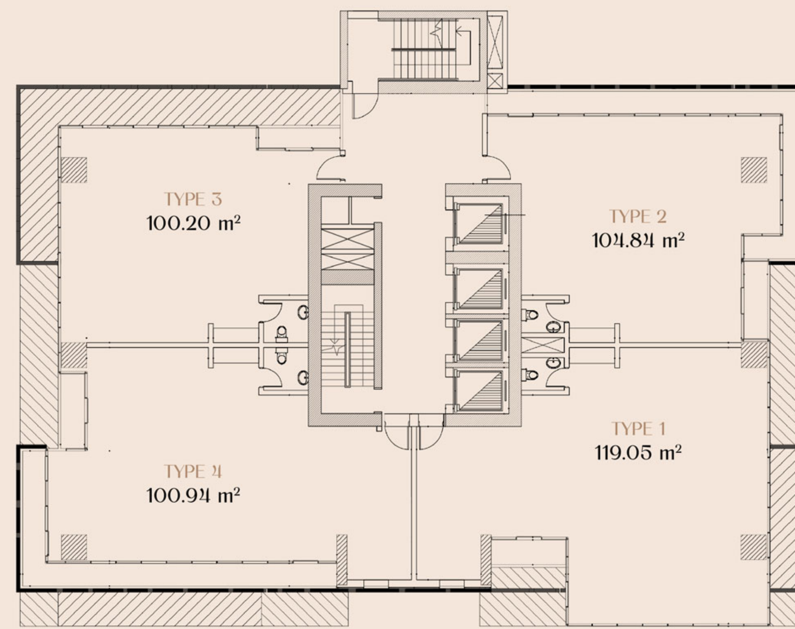
16 th , 18 th , 20 th FLOOR
