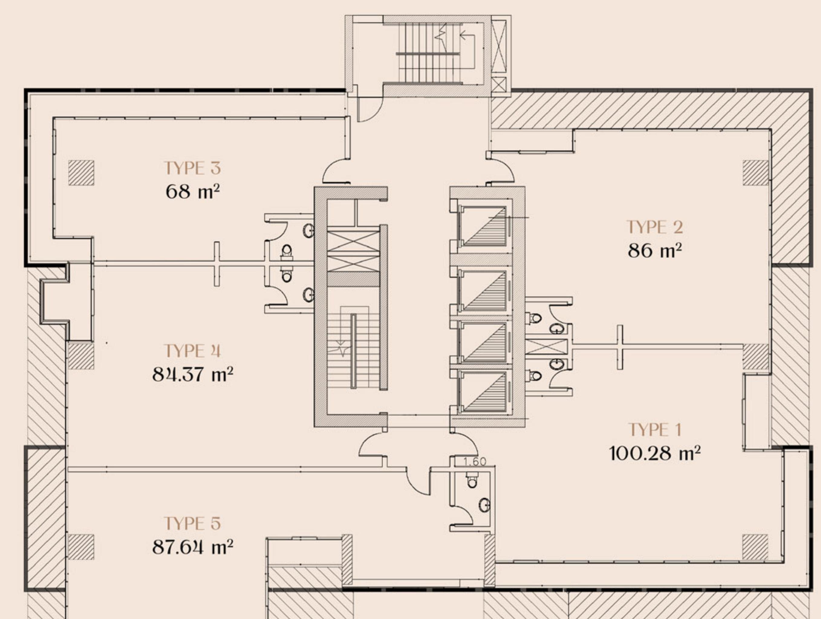
11 th , 12 th FLOOR
